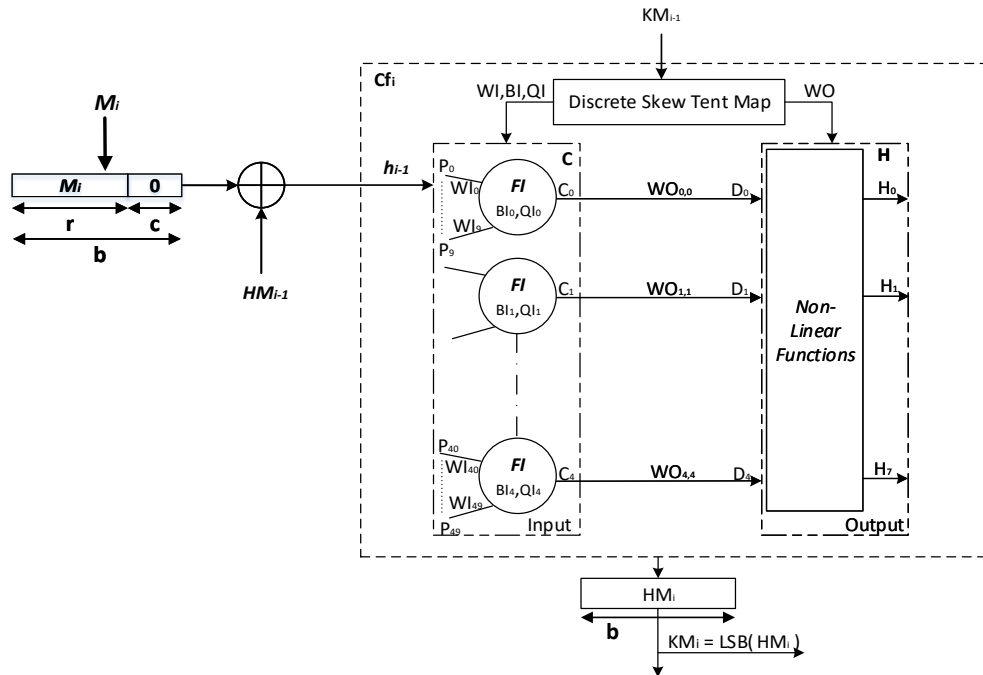
Figure 10. Detailed architecture of the i th chaotic function in the proposed keyed-Sponge hash function based on one-layered NL CNN.
