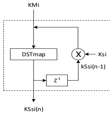
Figure 5. Structure of the i th Chaotic System used in the two proposed structure of keyed-Sponge CNN hash functions.
