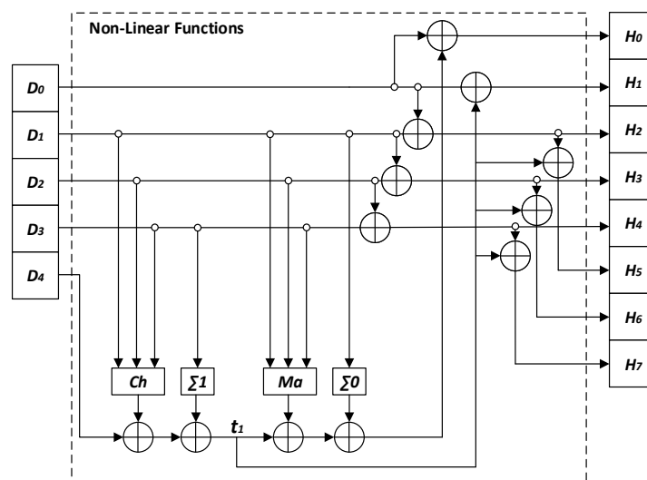
Figure 9. Detailed structure of NL Functions block.
